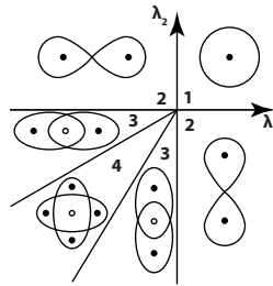
Figure 1: Bifurcation diagram
