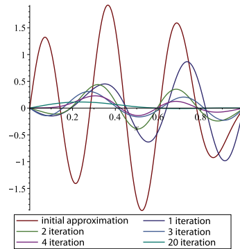
Figure 4: The initial value of the function and the first four and the twentieth iteration
