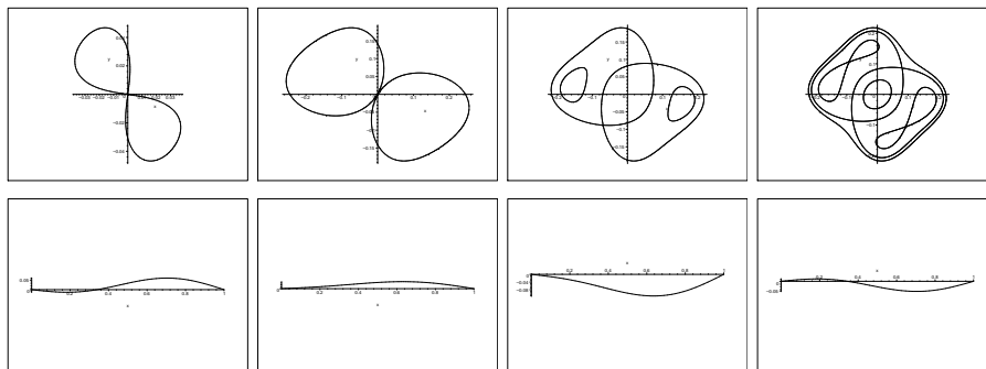
Figure 3: Contour curves and solutions
