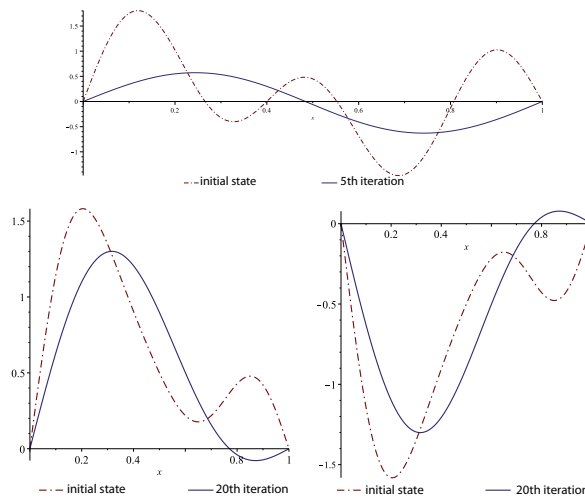
Figure 6: 1) Function f_1 ; 2) function f_2 ; 3) function f_3
