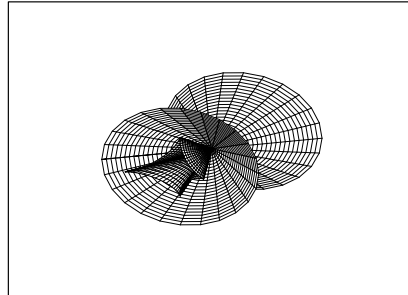
Figure 2: Caustic surface
