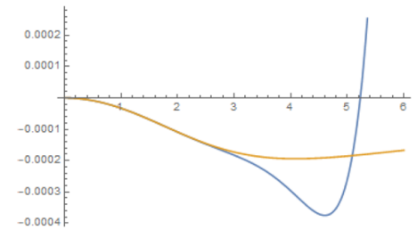
Figure 5: Plot of the V(t, t') function (blue line) and Padé approximation (orange line) for the metric Reissner-Nordström-de Sitter at M = 1 , r = 10 , Q = 1 , \Lambda = 1 .
